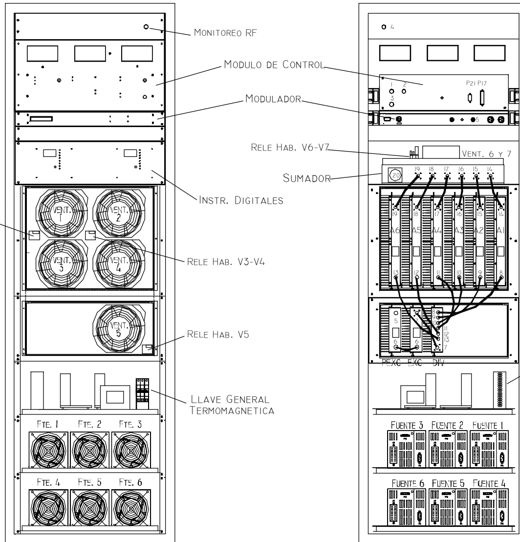
VISTA FRONTAL
